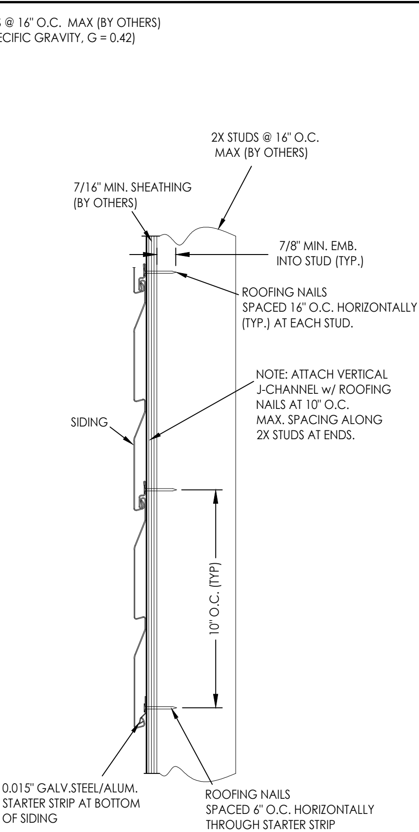
VERTICAL CROSS SECTION 2x stud construction w/ sheathing
