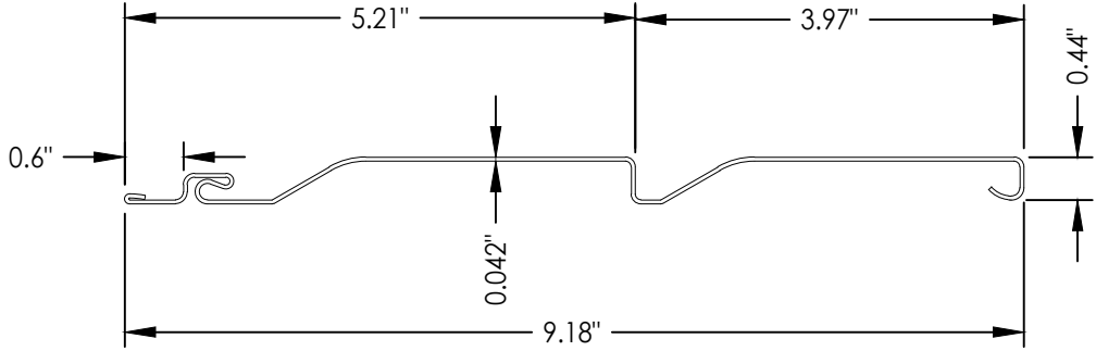
"COVENTRY" D4 DUTCH LAP
