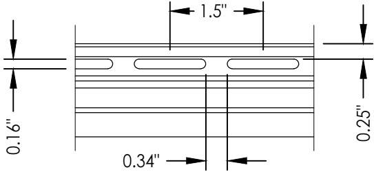
SIDING SLOT DETAILS
