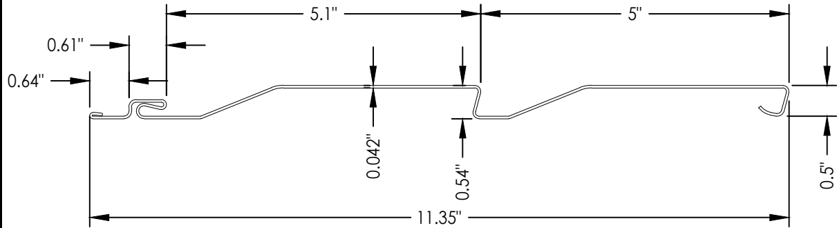
"COVENTRY" D5 DUTCH LAP
