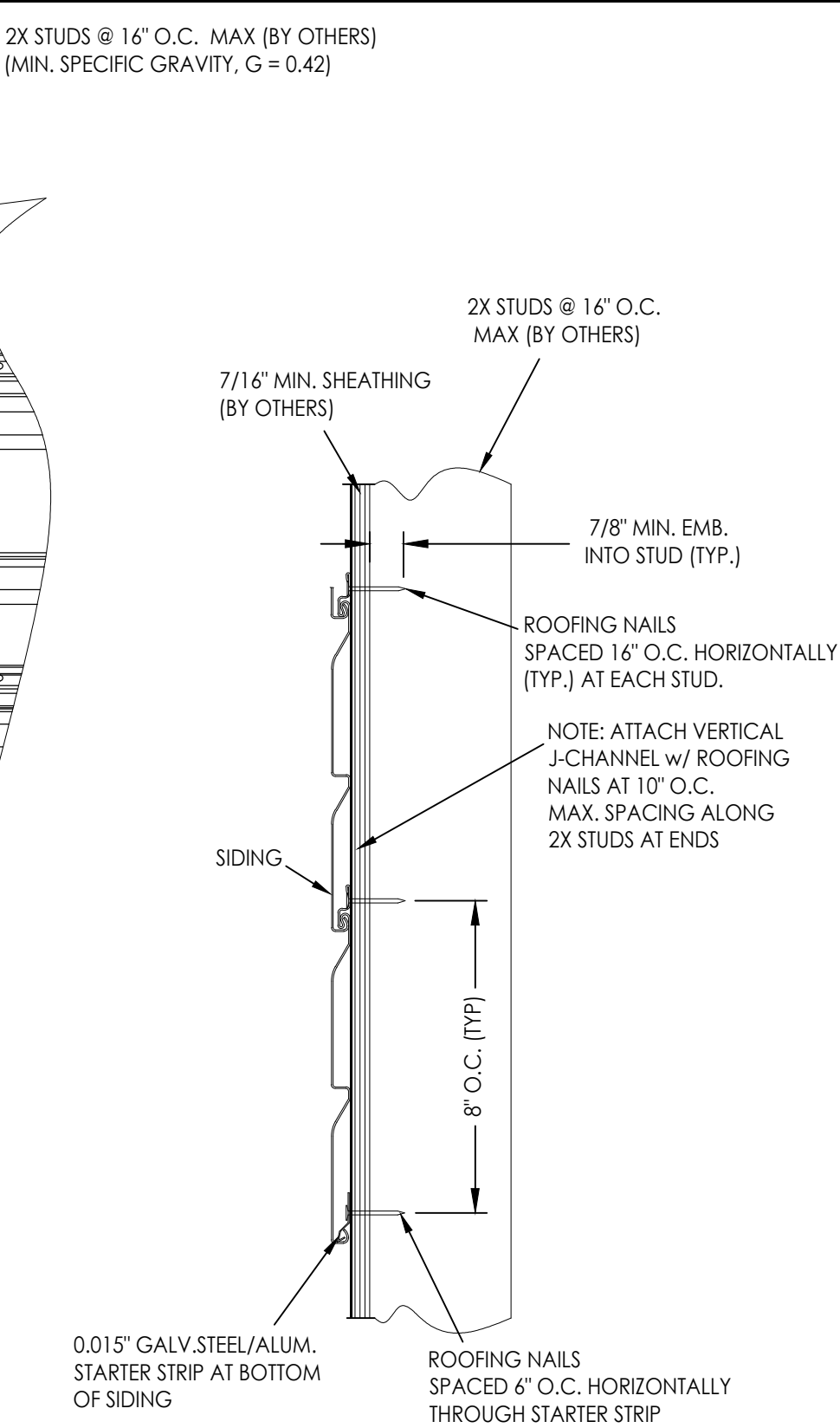
VERTICAL CROSS SECTION 2x stud construction w/ sheathing
